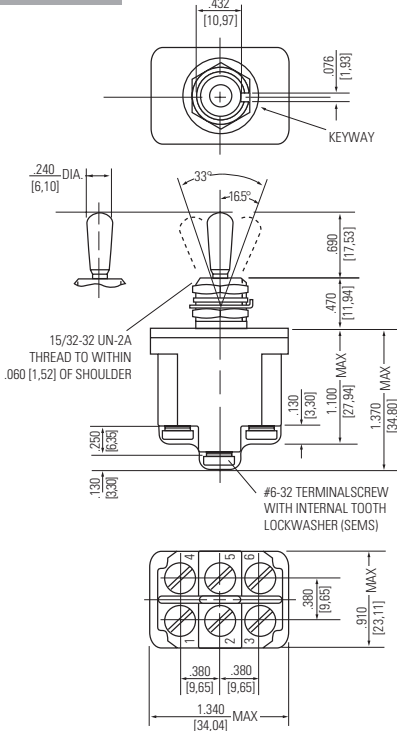
Terminal Identification
