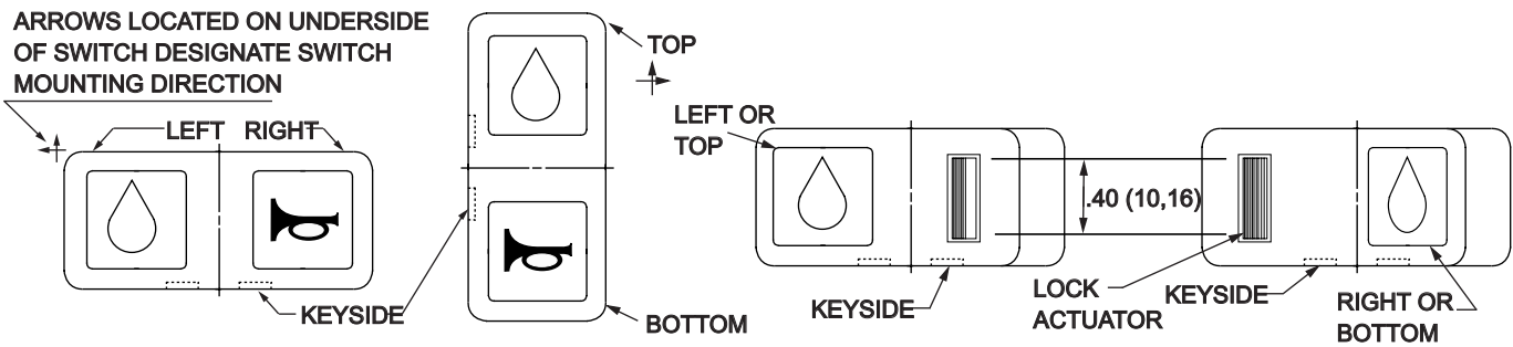
FIGURE 1 Horizontal Mount
