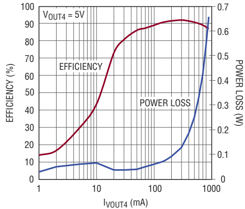
Boost Efficiency ( V_{IN4} = 3.8\text{V} )
