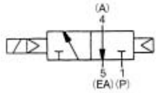
JIS Symbol Single solenoid
