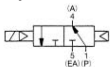
JIS Symbol Single solenoid
