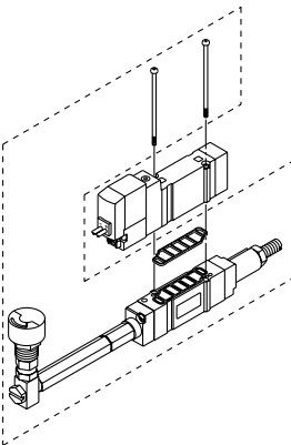
ARBY3000-06-□-2 (For even number stations)
