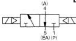
JIS Symbol Double solenoid
