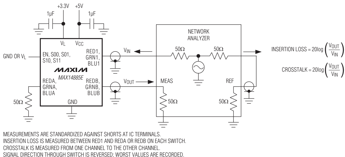
Figure 3. Insertion Loss and Crosstalk
