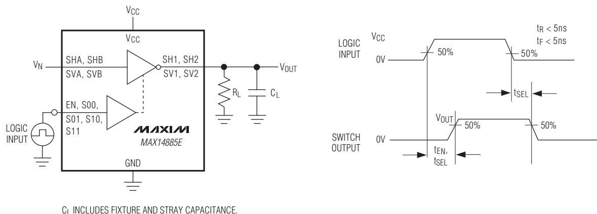
Figure 1. Enable/Select Time
