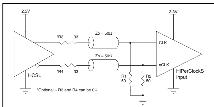
Figure 3E. HiPerClockS CLK/nCLK Input Driven by a 3.3V HCSTL Driver
