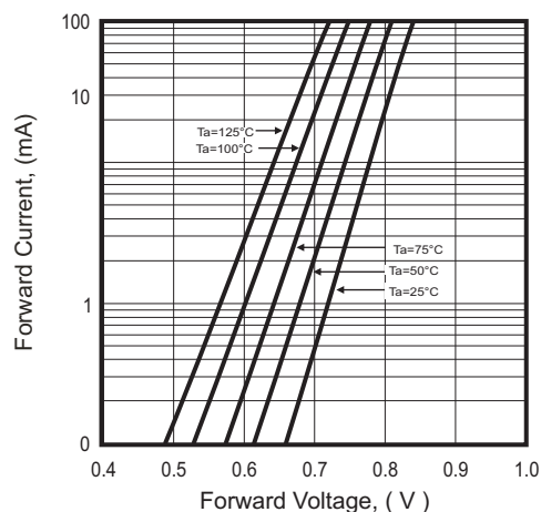
Fig.4 - Forward Characteristic
