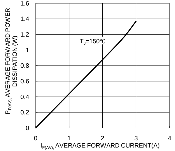
Figure 2. Forward Power Dissipation
