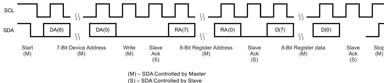
Figure 15. I²C Write
