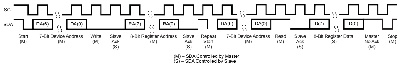
Figure 16. I²C Read
