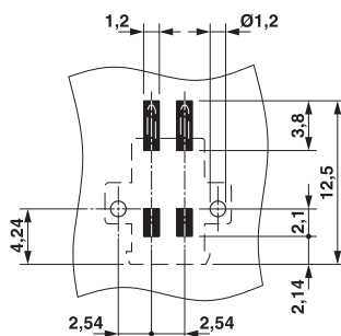
Drilling diagram
