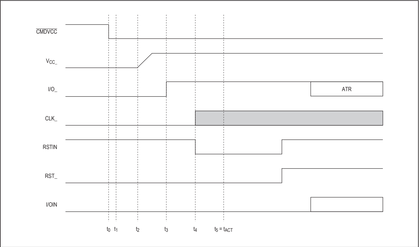
Figure 3. Activation Sequence Using \text{RSTIN} and \overline{\text{CMDVCC}}
