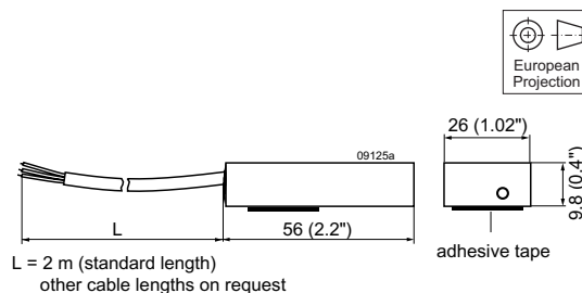
Fig. 46 Battery temperature sensor
