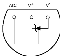
TO92 (Bottom view)
