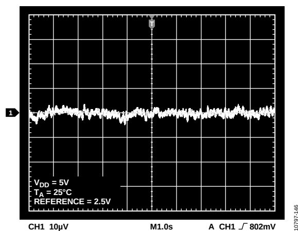
Figure 32. 0.1 Hz to 10 Hz Output Noise Plot
