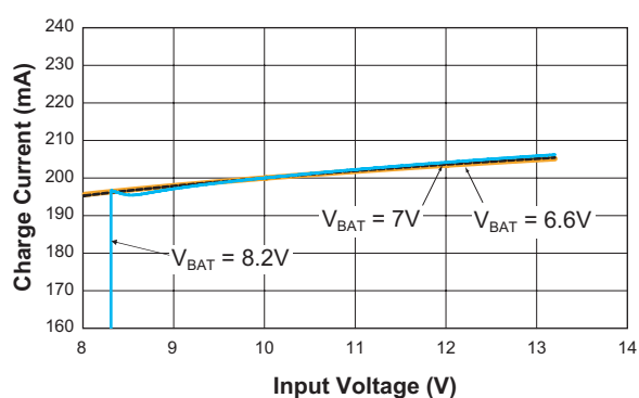
Constant Charge Current vs. Input Voltage ( R_{SET} = 8.87K\Omega )
