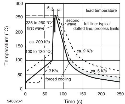
Figure 12. Double Wave Soldering of Opto Devices (all Packages)
