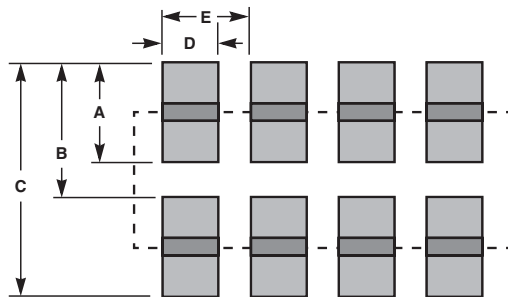
PAD LAYOUT DIMENSIONS
