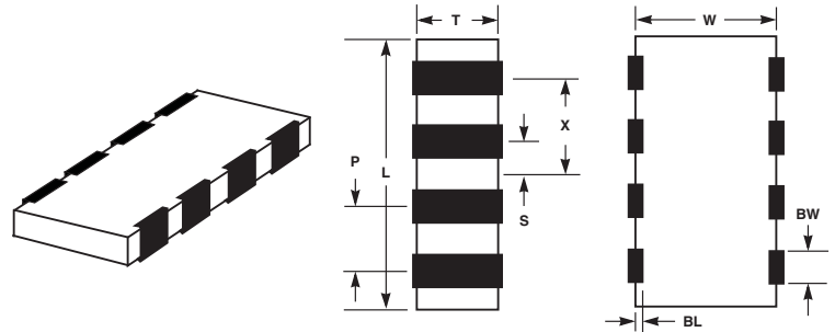
CHIP LAYOUT DIMENSIONS
