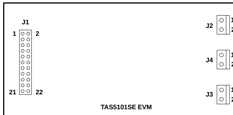
Figure 1–1. Connector Diagram
