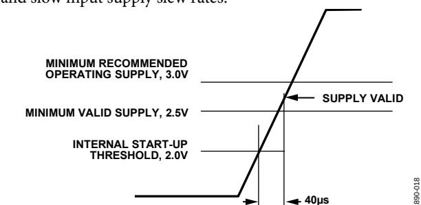
Figure 18. Digital Isolator Start-Up Condition, Supply Slew Rate > 12.5 V/ms
