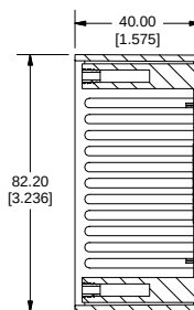
SECTION B-B
