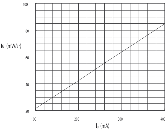
Figure 3. I_F - I_e Characteristics ( 0^\circ )
