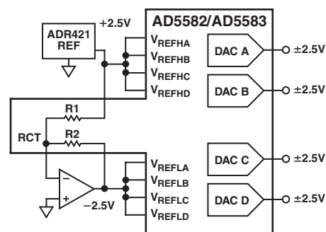
Figure 1. Using Built-In Matching Resistors to Generate a Negative Voltage Reference
