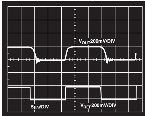
TPC 20. Small Signal Response Operating at Near Rail, C_L = 2 nF (See Test Circuit 1)
