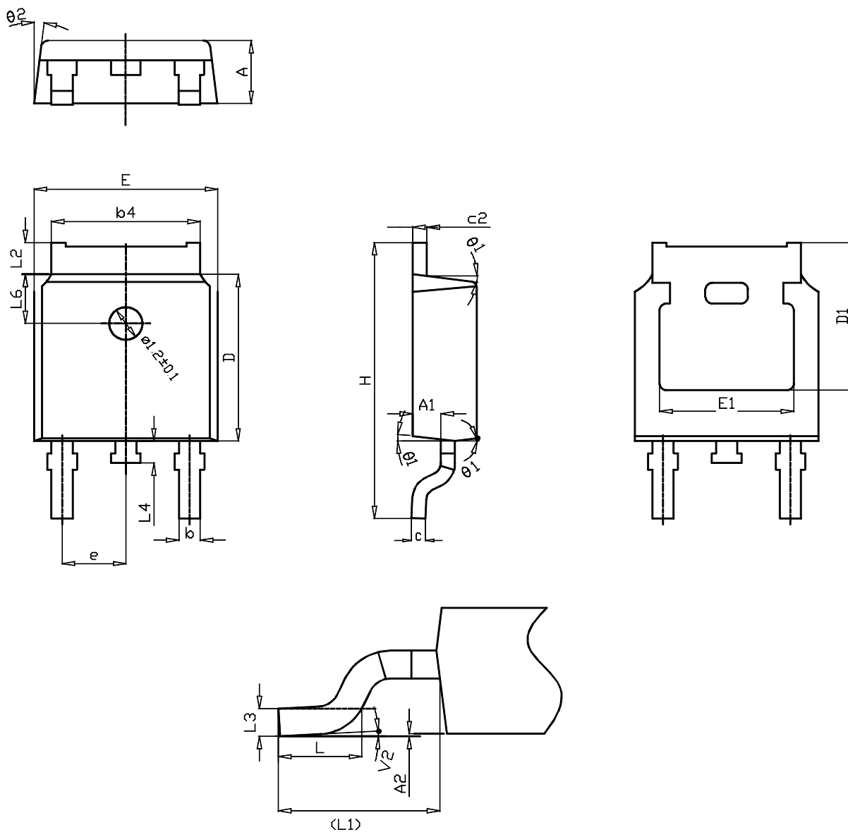
Figure 22. DPAK (TO-252) type C package outline
