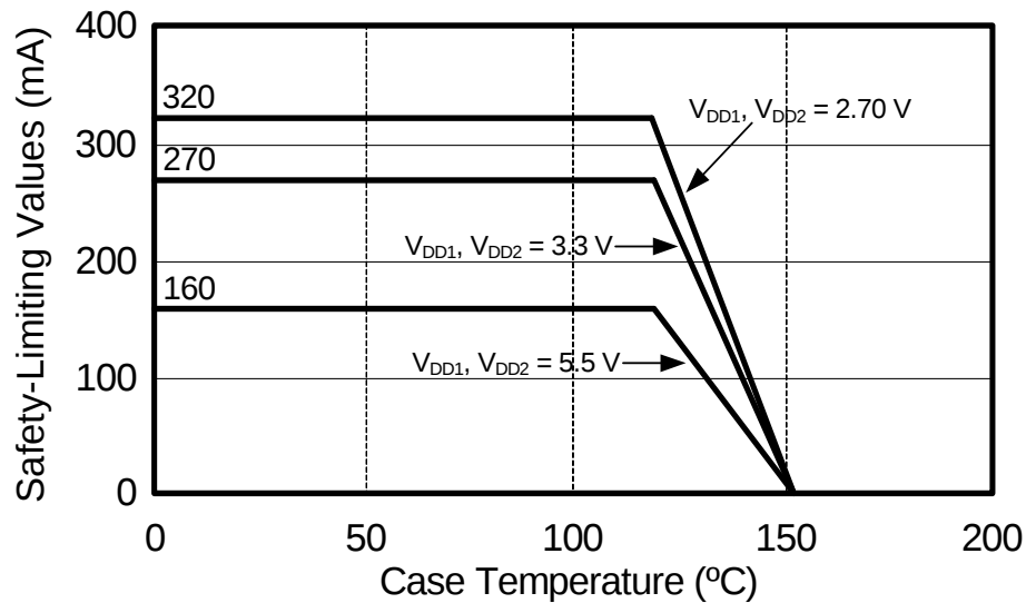
Figure 3. (NB SOIC-8) Thermal Derating Curve, Dependence of Safety Limiting Values with Case Temperature per DIN EN 60747-5-5
