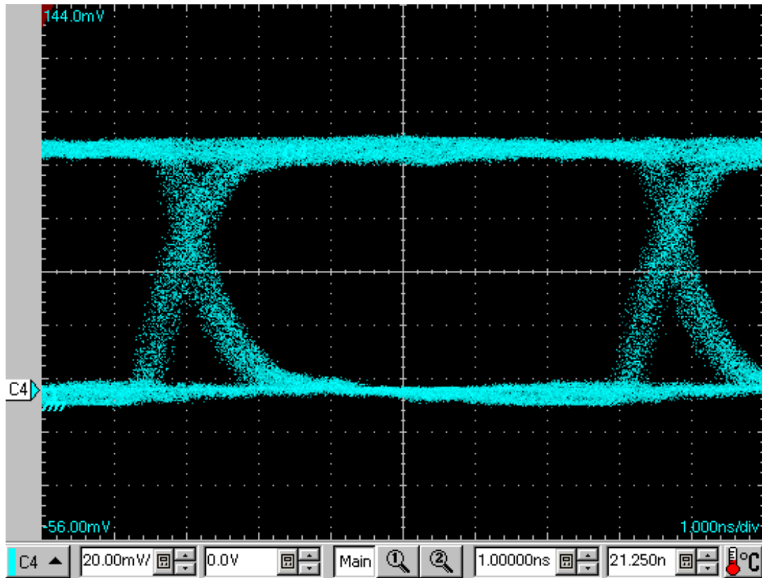
Figure 6. Eye Diagram
