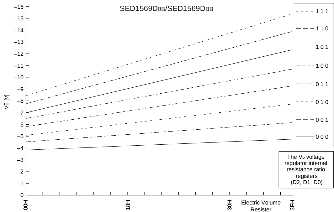
Figure 19: SED1569D0B/SED1569D8B (Temperature Gradient = -0.05%/°C Model)
