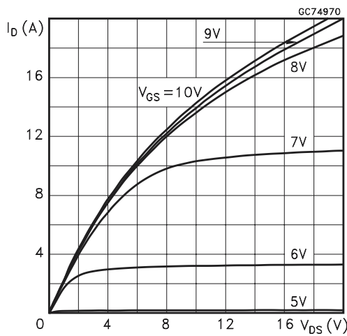
Figure 5. Output Characteristics
