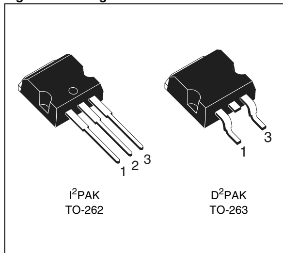
Figure 1. Package
