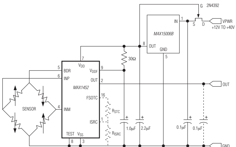
Figure 3. Basic Nonratiometric Output Configuration
