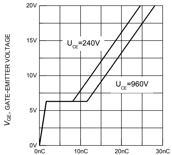
Figure 19. Typical gate charge ( I_C = 3A )
