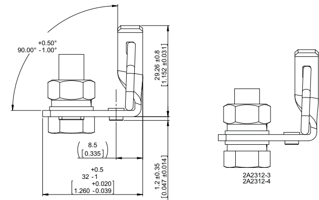
Clinch nut
