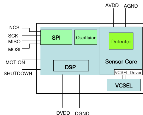
Figure 2. CYONS1001L Chip
