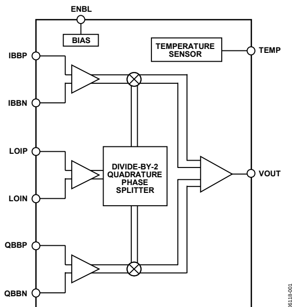
Figure 26. ADL5385 Block Diagram
