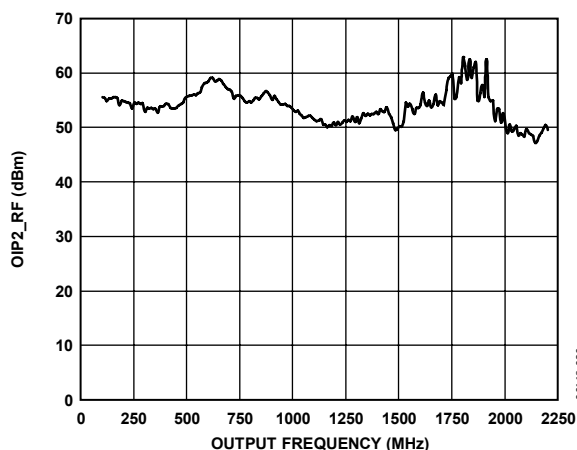
Figure 40. Output Second-Order Intermodulation vs. Carrier Frequency
