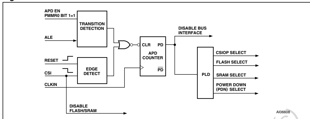
Figure 67. APD unit
