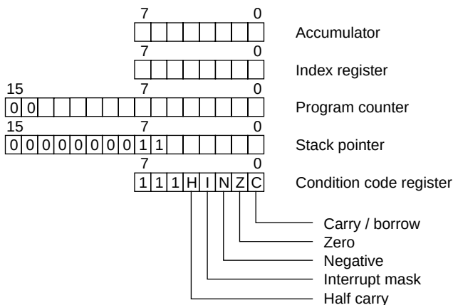
Figure 11-1 Programming model
