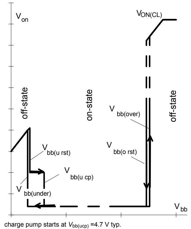
Figure 7a: Overvoltage:
