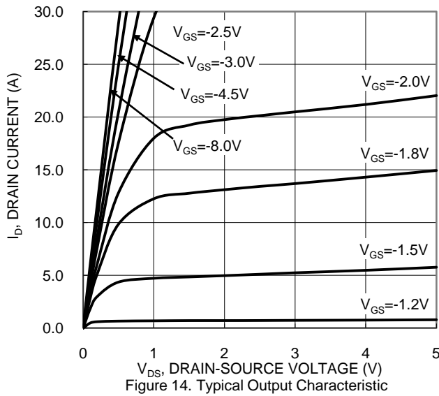
Figure 14. Typical Output Characteristic
