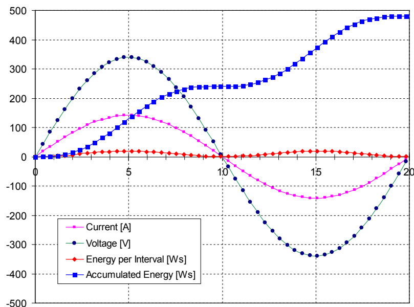
Figure 5: Voltage, Current, Momentary and Accumulated Energy
