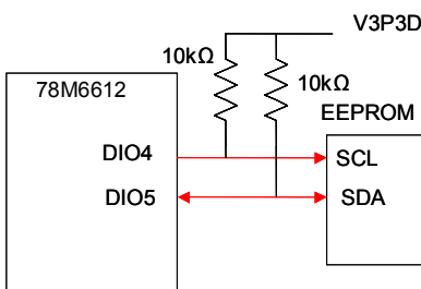
Figure 12: I 2 C EEPROM Connection
