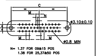
PCB DRILLING DETAIL - 50 POS
