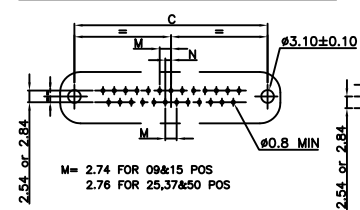
PCB DRILLING DETAIL - 09 TO 37 POS
