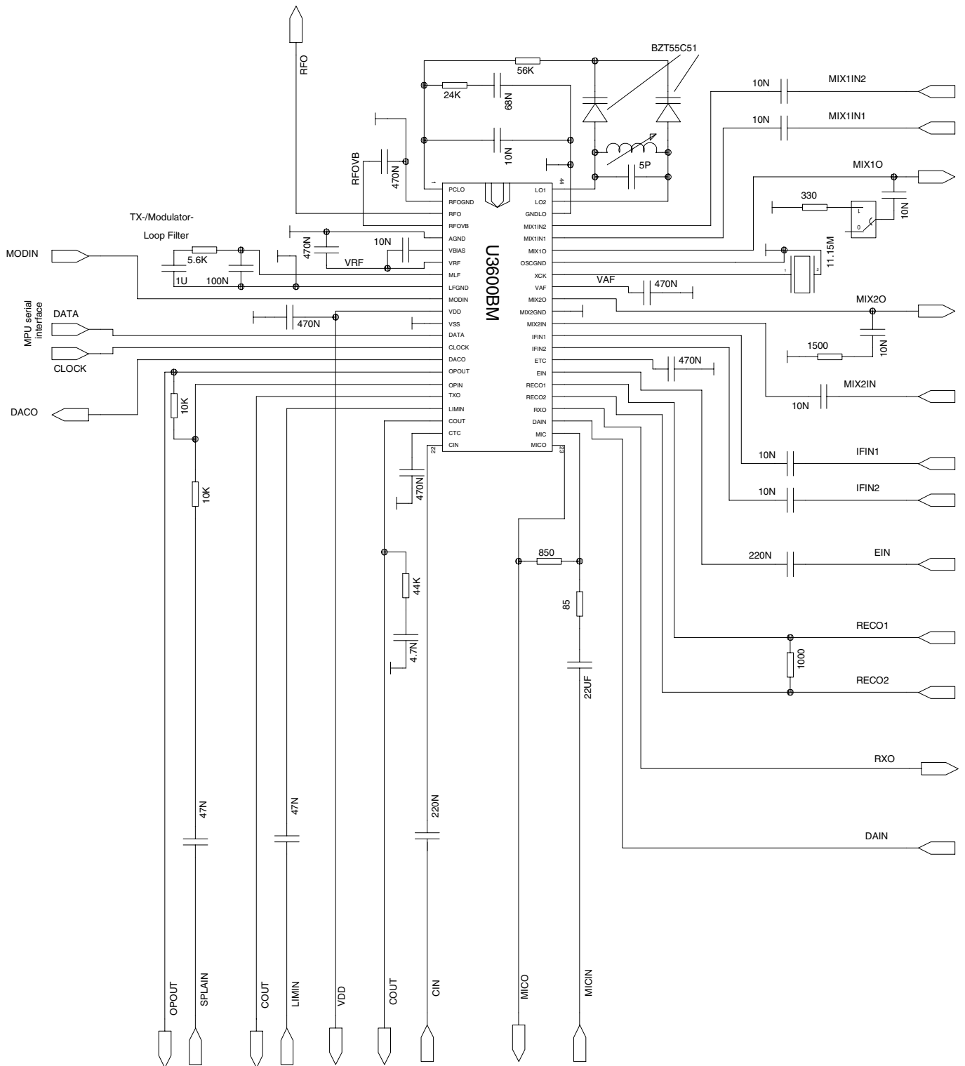
Figure 8-1. Test Circuit
