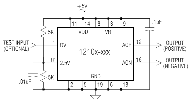
RECOMMENDED CONNECTIONS
