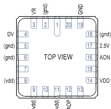
PINOUT
