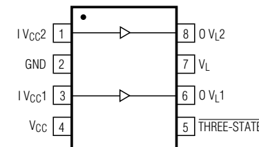
TDFN-8 (3mm x 3mm) TOP VIEW
