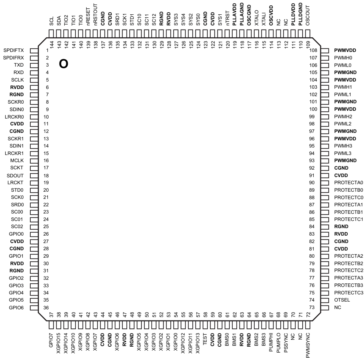
D2-1 Family (144 LD LQFP) TOP VIEW
