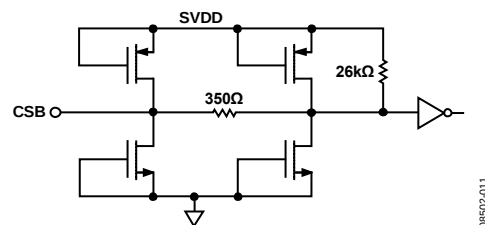
Figure 60. Equivalent CSB Input Circuit
