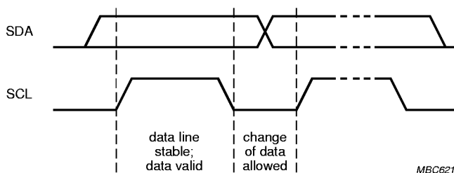
Fig.4 Bit transfer.
