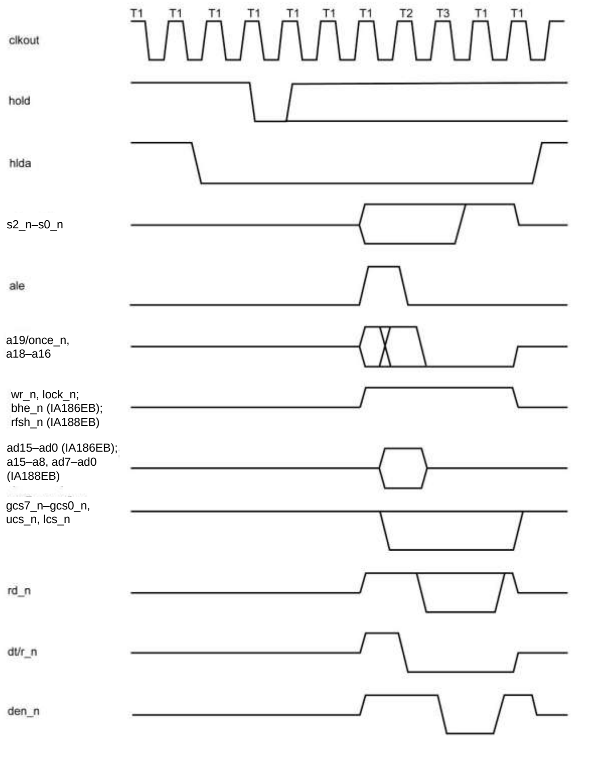
Figure 25. Refresh During Hold Acknowledge Timing
