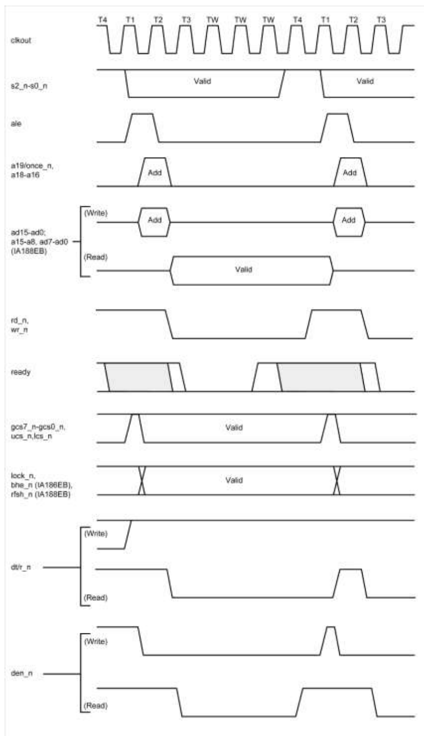
Figure 26. Ready Timing
