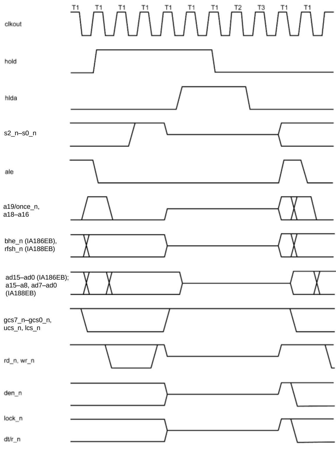
Figure 24. hold/hlda Timing
