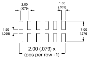
Recommended PCB layouts
