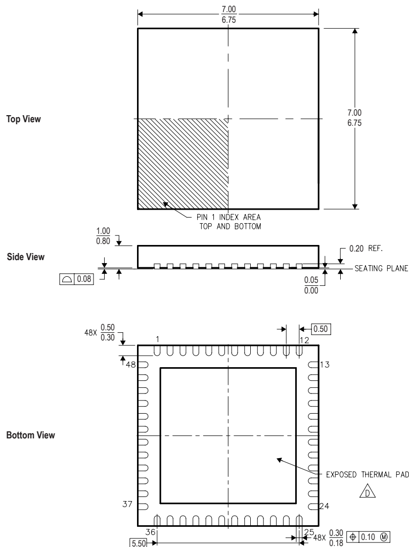
Figure D-4. Stellaris LM3S608 48-Pin QFN Package
