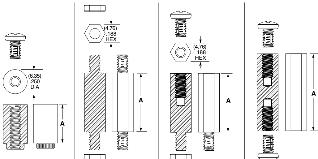
-01 LEAD STYLE
