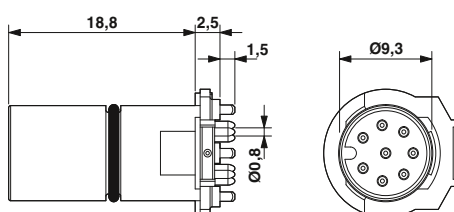
M12 plug contact carrier, straight, 8-pos.
