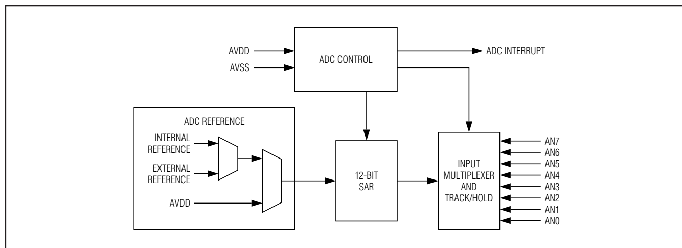
Figure 7. ADC Block Diagram
