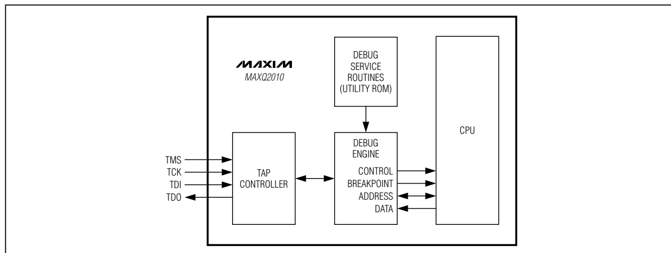
Figure 9. In-Circuit Debugger
