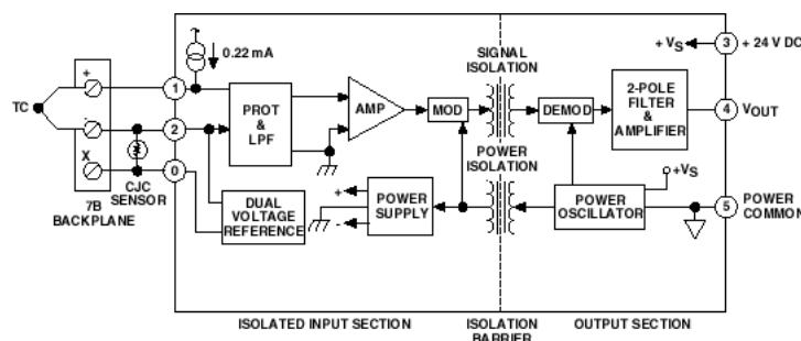
Figure 1. 7B37 Functional Block Diagram
