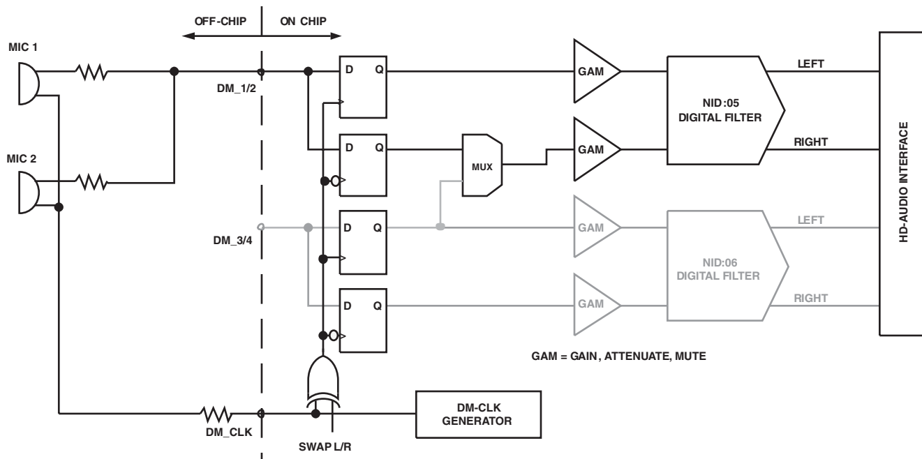
Figure 6. Multiplex Digital Microphone, Stereo Interface
